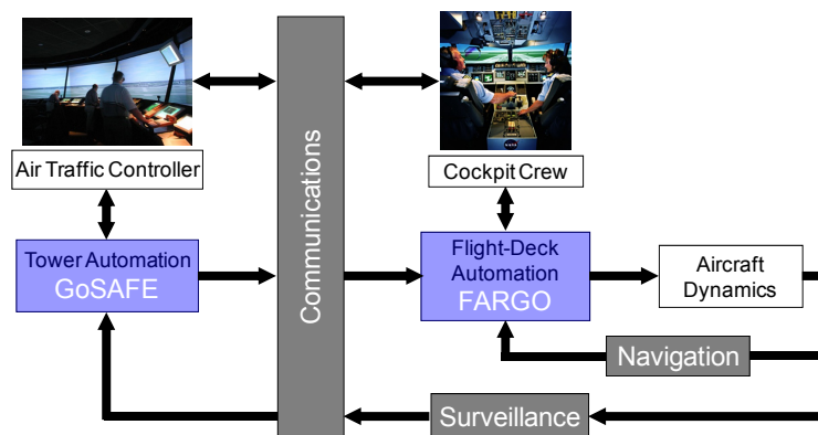
Figure 3. Block Diagram of SOAR Concept.
