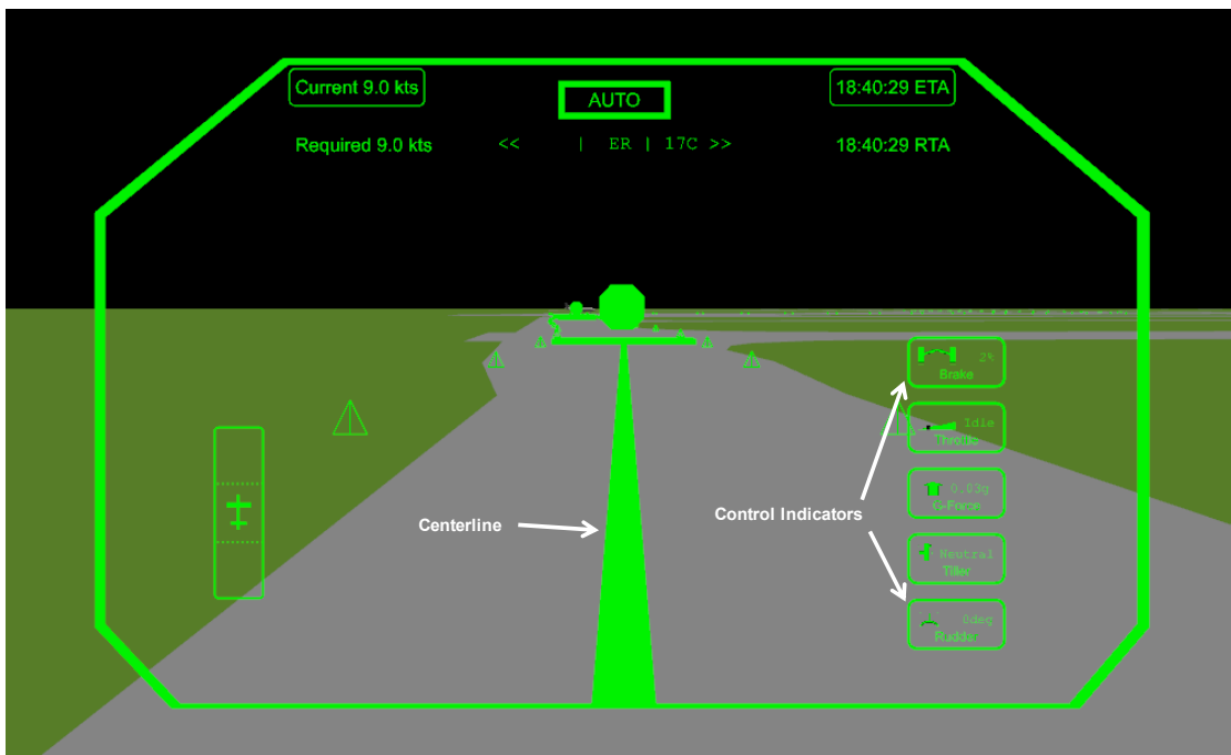
Figure 13. Sample HUD Display for Auto-Taxi Mode.
