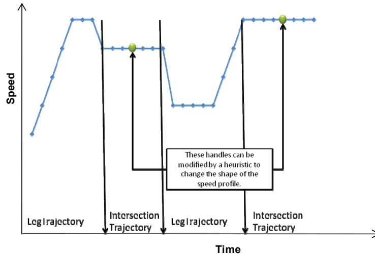
Figure 9. Definition of Speed Profile for 4D Trajectory.
