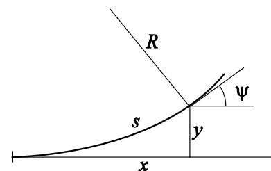
Figure 8. Transition Spiral.
