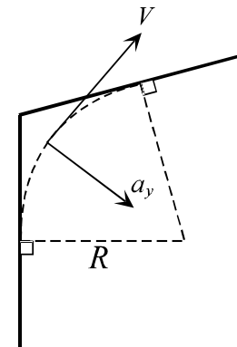
Figure 7. Turn Arc between Connected Linear Segments.
