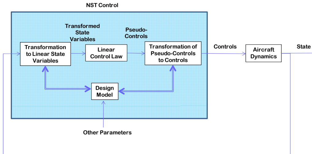
Figure 10. Concept of Nonlinear Controller Based on Feedback Linearization.
