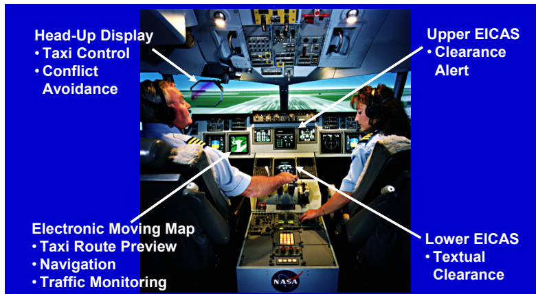
Figure 6. FARGO Pilot-Interface Displays.
