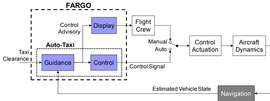
Figure 4. General Block Diagram of FARGO Concept.
