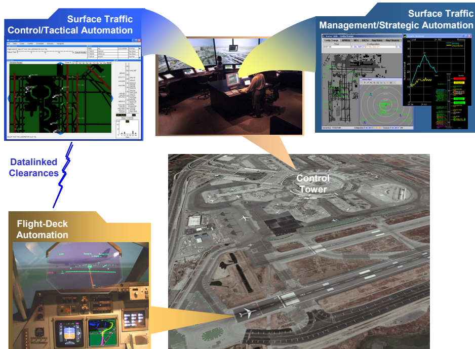
Figure 2. Collaborative Automation between Tower and Flight Deck Operations.
