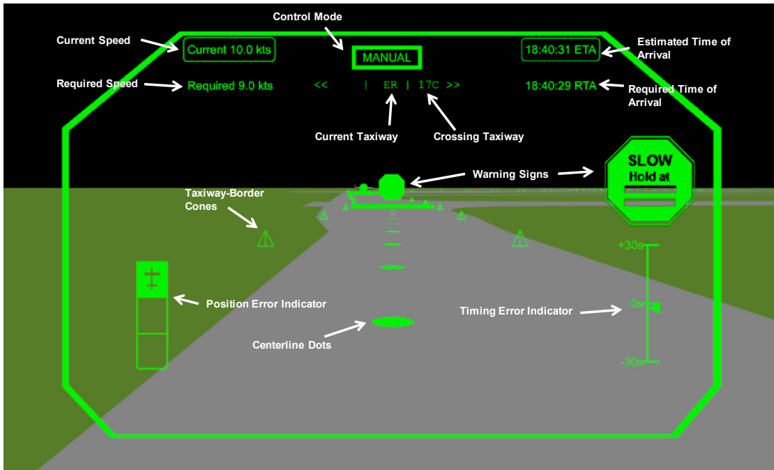
Figure 12. Sample HUD Display for Manual Control Mode.
