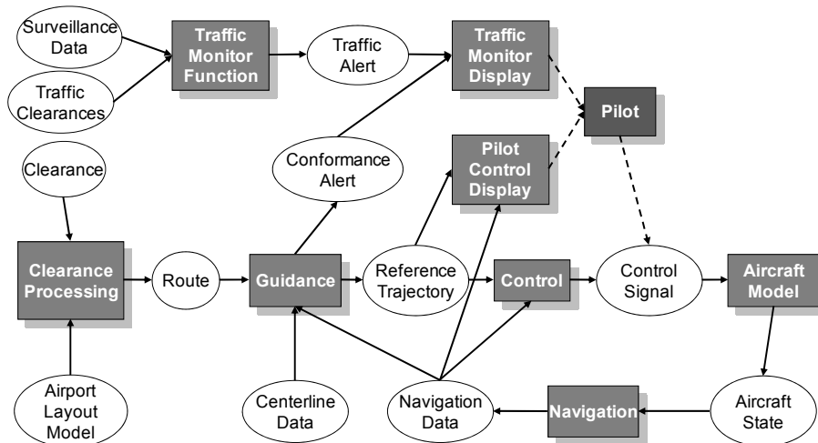
Figure 5. Data Flow Diagram of FARGO Processes.
